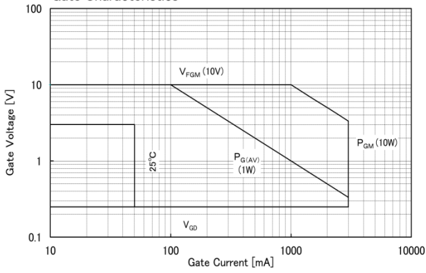
Gate Characteristics
